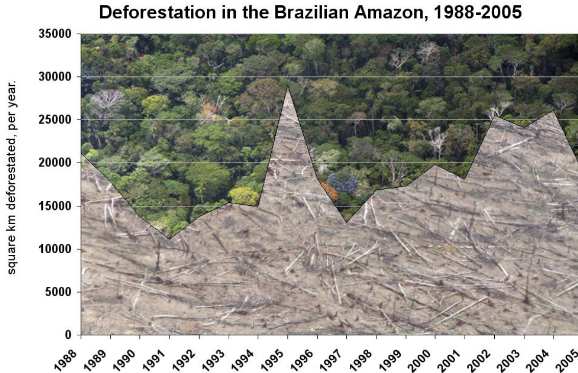
Fig. 4. Deforestation rates in Brazilian Amazonia (INPE).
