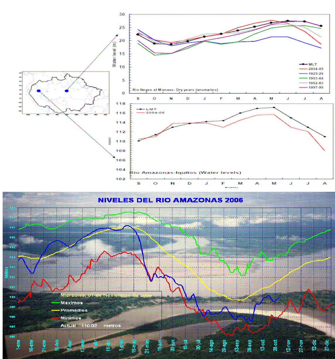
Fig. 11. Upper panel: Levels of the Rio Negro at Manaus during some drought years in Amazonia (2004-2005, 1925-26, 1963-64, 1982-83, 1997-98) and of the Rio Amazonas in Iquitos during 2005 (Marengo et al. 2006). Lower panel: Levels of the Amazon River at Iquitos during 2006 (source: www.dhn.mil.pe )
