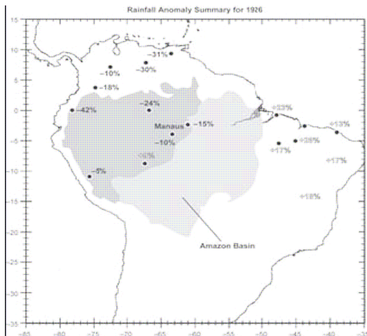
Fig. 9 - Summary of the annual (January-December) rainfall anomaly for the dry year of 1926 over South America for all stations available in this study. An east-west dipole is apparent, with reduced rainfall upstream from Manaus and enhanced rainfall further east and extending to the Nordeste region (Williams et al. 2005).
