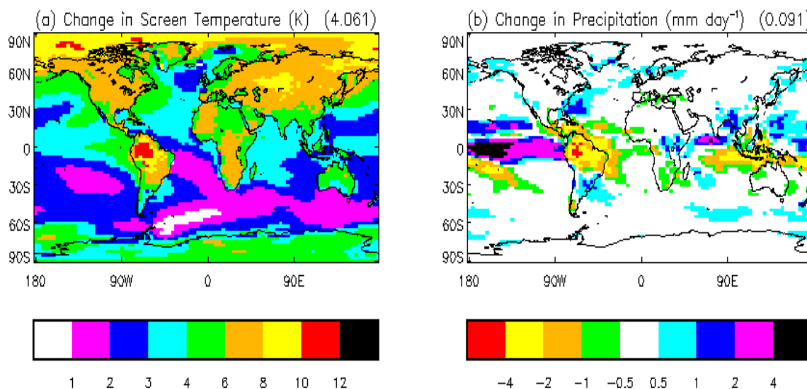
Fig. 3. Change in Global Climate in HadCM3LC Interactive CO 2 and Dynamic Vegetation, for surface temperature (left, in °C) and rainfall (right, in mm/day). Maps show the difference between 2090-2100 and 1980-1990. (Cox et al 2000, 2004)
