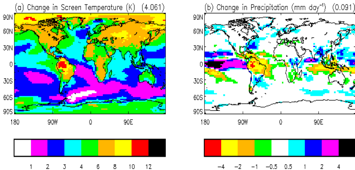
Fig. 2. Change in Global Climate in HadCM3LC Interactive CO 2 and Dynamic Vegetation, for surface temperature (left, in °C) and rainfall (right, in mm/day). Maps show the difference between 2090-2100 and 1980-1990. (Cox et al 2000, 2004)
