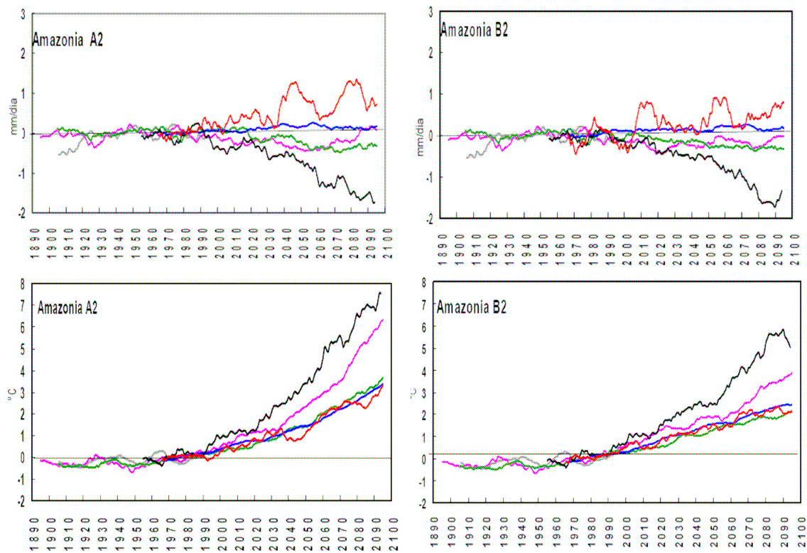
Fig. 1. Time series of rainfall and air temperatures anomalies for the Amazon region from 1890 to 2100. The anomalies are calculated based on the 1961-90 climatology from five IPCC TAR models (CCCMA, CCSR/NIES, CSIRO, GFDL and HadCM3) and observations from the CRU. Scenarios are A2 (high) and B2 (low) emission scenarios. The lines represent the 11-year moving average of each time series. Color lines indicate the different models used (Marengo 2006b).
