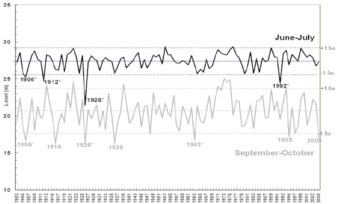
Fig. 8. Negro River water levels at Manaus (in m) in the Manaus station, Brazil, during the peak water level season in June-July (black lines) and the low water level season in September-October (grey lines). Full/thin broken lines represent the mean/+ 1.5 \sigma . The number indicates years where the levels reached values lower than 1.5 \sigma . Asterisks depict El Niño years (Marengo et al. 2006).
