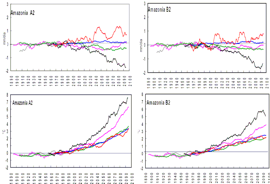
Fig. 2. Time series of rainfall and air temperatures anomalies for the Amazon region from 1890 to 2100. The anomalies are calculated based on the 1961-90 climatology from five IPCC TAR models (CCCMA, CCSR/NIES, CSIRO, GFDL and HadCM3) and observations from the CRU. Scenarios are A2 (high) and B2 (low) emission scenarios. The lines represent the 11-year moving average of each time series. Color lines indicate the different models used (Marengo 2006b).
