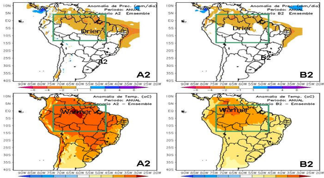
Fig. 3. Projected changes in annual rainfall and air temperature anomalies for the Scenarios A2 (Left) and B2 (right). Units are mm/day (rainfall) and (°C) for temperatures. Results are the ensemble of 3 regional models (Eta/CPTEC, RegCM3 and HadRM3P) for the period 2071-2100 relative to 1961-90. Green square represents the Amazon region (Source: Ambrizzi et al. 2006).
