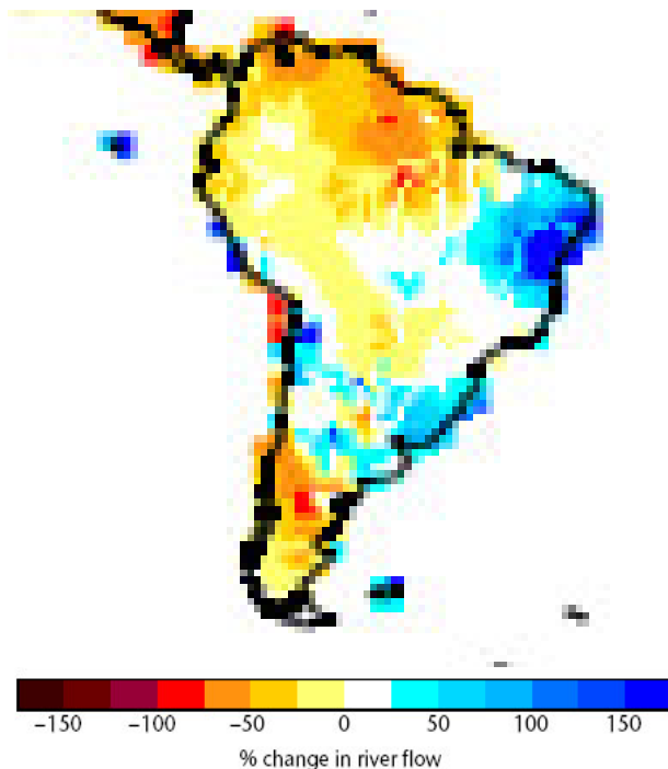
Fig. 5. River flow changes (%) in South America for 2061-2100 relative to 1901-1998. Scenario A1B, HadGEM1 model (UK Met Office 2005).
