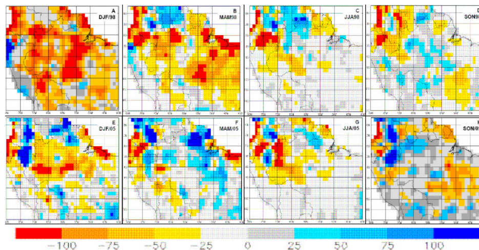
Fig. 12. Seasonal rainfall maps for tropical South America during two drought events: 1998 (upper panels), and 2005 (lower panel). Values are shown as deviations from the 1961-1990 long-term mean. Data is from GPCC. Units are in mm/month (Marengo et al. 2006)
