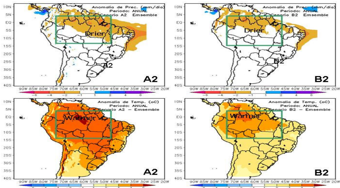
Fig. 13. Projected changes in annual rainfall and air temperature anomalies for the Scenarios A2 (Left) and B2 (right). Units are mm/day (rainfall) and (°C) for temperatures. Results are the ensemble of 3 regional models (Eta/CPTEC,
