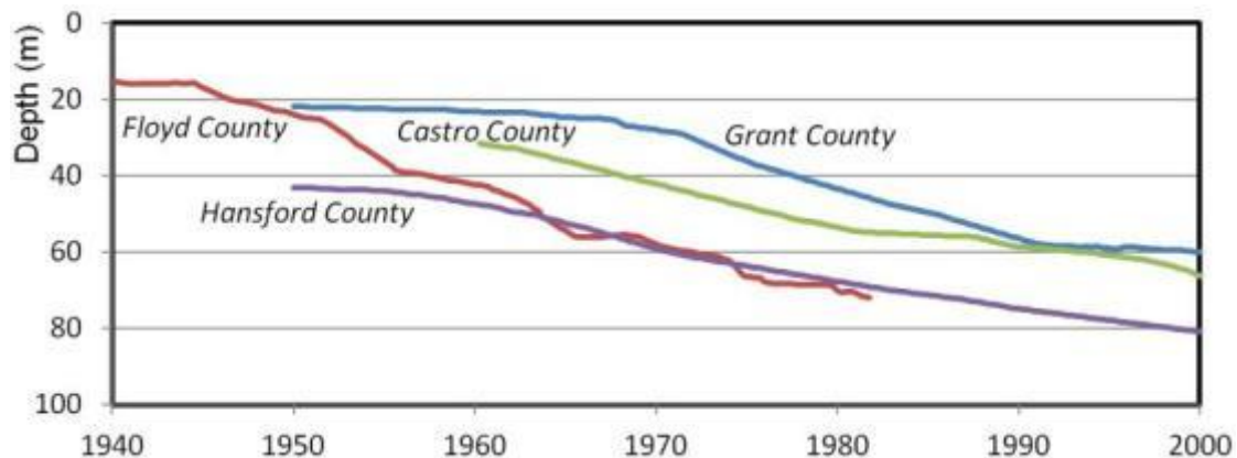
Figure 2.10 Example of long-term declines of groundwater levels: unprecedented change in groundwater state on the High Plains, USA (Margat & Van der Gun, 2013)
