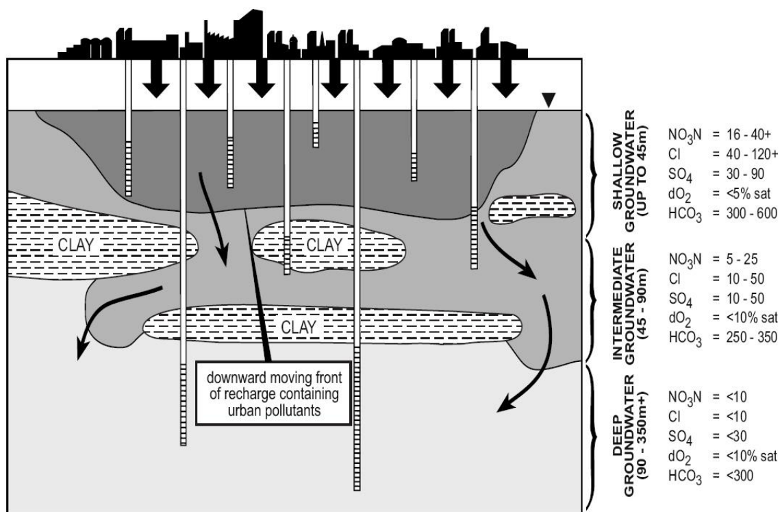
Figure 2.11 Stratification of diffuse urban pollution below the Bolivian city of Santa Cruz (Chilton, 2006)
