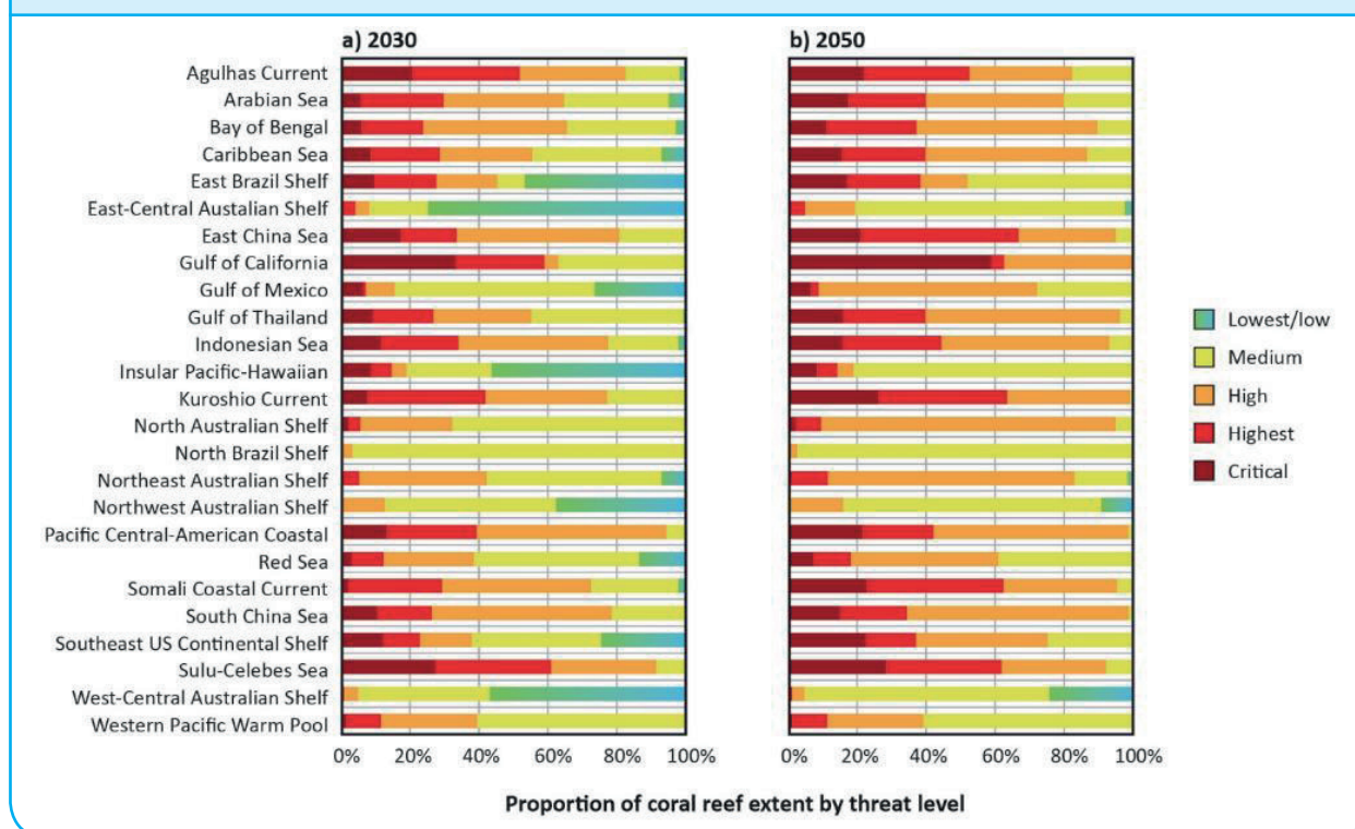
Summary Figure 11 Projected proportion of LMEs and WPWP coral reef area by threat level for global threats (warming and acidification) by a) 2030 and b) 2050
