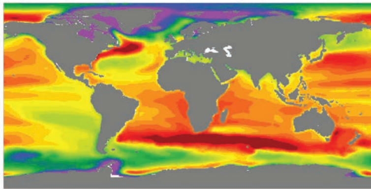
b) Sea-level Rise Threat Index in 2100 for SSP3
