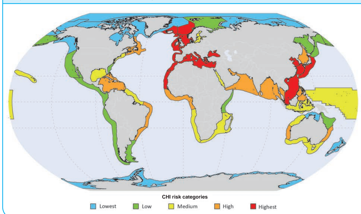
Figure 7.28 Cumulative human impact risk categories of LMEs and the WPWP. LMEs are ranked by the average cumulative human impact scores across the entire region. LMEs in Europe, Northern Africa, and Southeast Asia are at highest risk.
