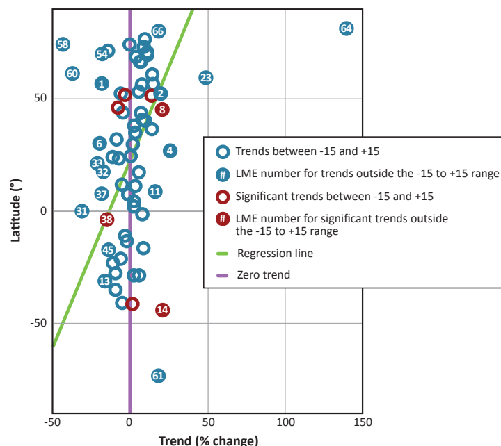
Figure 5.5 Trends in chlorophyll a (2003–2013) in relation to latitude. No large-scale, consistent pattern of either increase or decrease in chlorophyll a was observed. There are 36 LMEs with positive chlorophyll a trends and 31 with negative chlorophyll a trends, and trends are weakly correlated with latitude. The four LMEs with statistically significant increasing chlorophyll a trends (red circles to the right of the purple line) are the Scotian Shelf (#8), Patagonian Shelf (#14), Newfoundland-Labrador Shelf, and Southeast Australian Shelf. The three LMEs with statistically significant decreasing chlorophyll a trends (red circles to the left of the purple line) are the Indonesian Sea (#38), Oyashio Current, and Celtic-Biscay Shelf.
