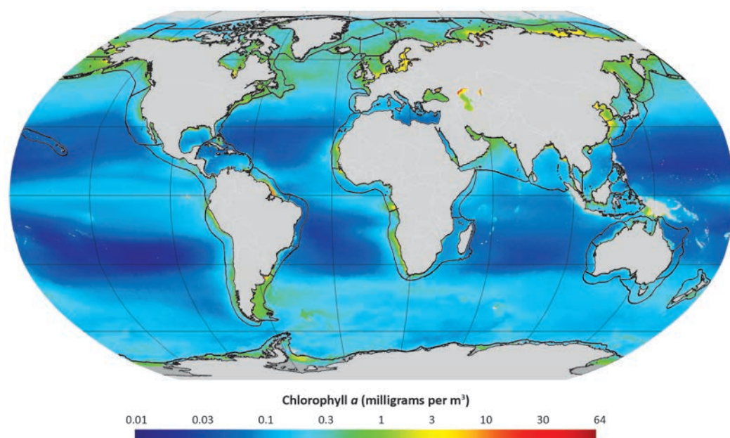
Figure 5.1 Distribution of average surface chlorophyll a throughout the global ocean, 1998–2013. Mean concentrations of chlorophyll a , the green pigment involved in photosynthesis and an index of phytoplankton abundance, vary from 0.008 to 100 milligrams per m 3 , a range of more than four orders of magnitude. The highest values are found near shore, within LME boundaries.
