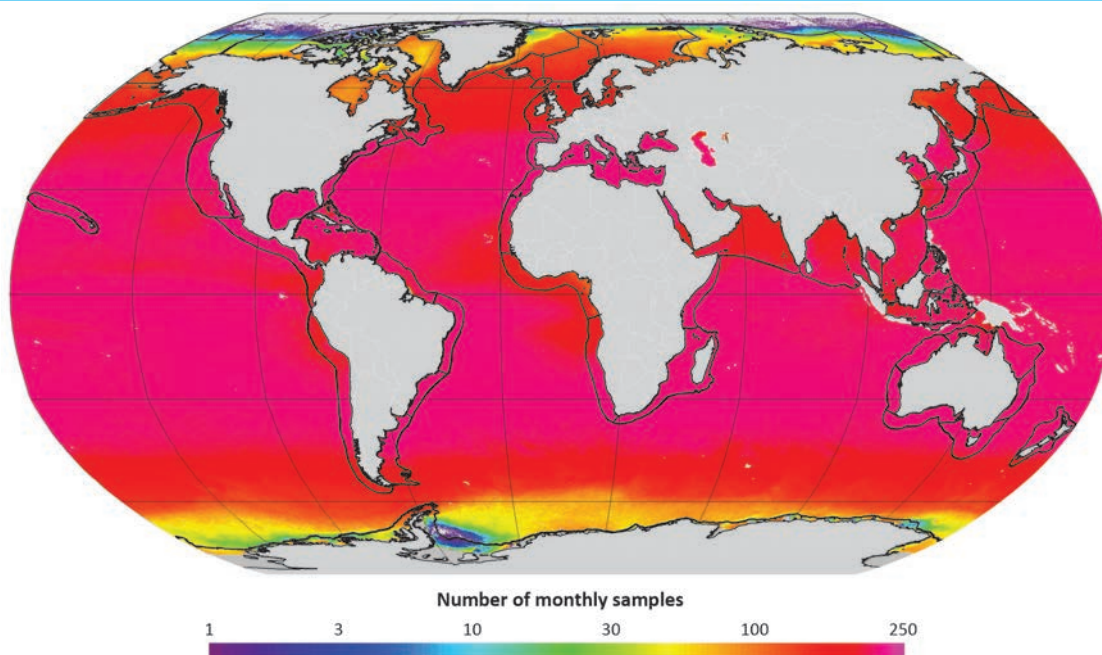
Figure 5.6 Global distribution of chlorophyll a samples, 1998–2013. The confidence level of the primary productivity estimates is high where sampling is adequate, which is the case for most LMEs. However, sampling by satellite ocean colour sensors was inadequate for a comprehensive characterization of chlorophyll a and primary productivity in northern and southern LMEs with short growing seasons, persistent ice or clouds, and partial coverage by satellite sensors that rely on daylight for ocean colour measurements.
