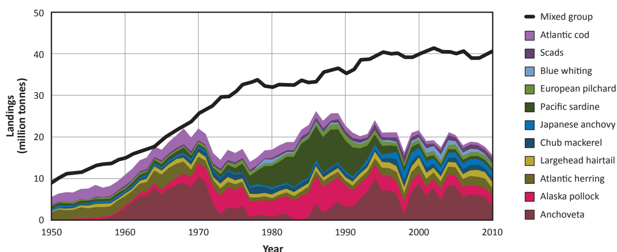
Figure 6.1 Time series of landings by species in all LMEs, 1950–2010
