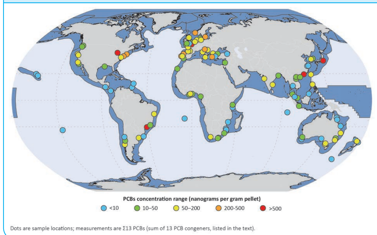
Figure 7.8 Concentrations of PCBs in beached plastic pellets within LMEs. Legacy pollution, where bottom sediments act as secondary sources of contamination, is observed in urban coastal waters in Western Europe, the US east and west coasts, and Japan. Results suggest current or recent inputs of PCBs for some developing countries such as Ghana and the Philippines.
