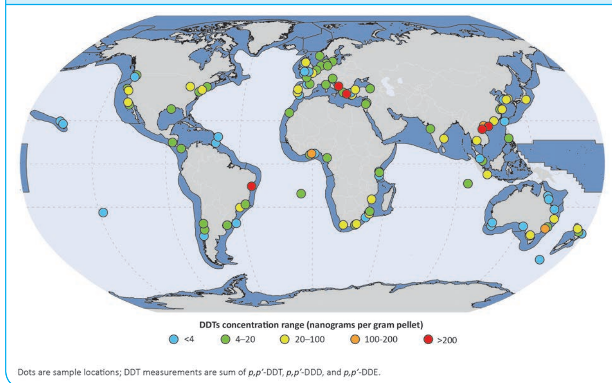
Figure 7.9 Concentrations of DDTs in beached plastic pellets within LMEs. Legacy pollution is observed in areas where DDT pesticide was used for agricultural production. For some tropical countries, there is evidence of current and/or recent inputs of DDT used for malaria control.
