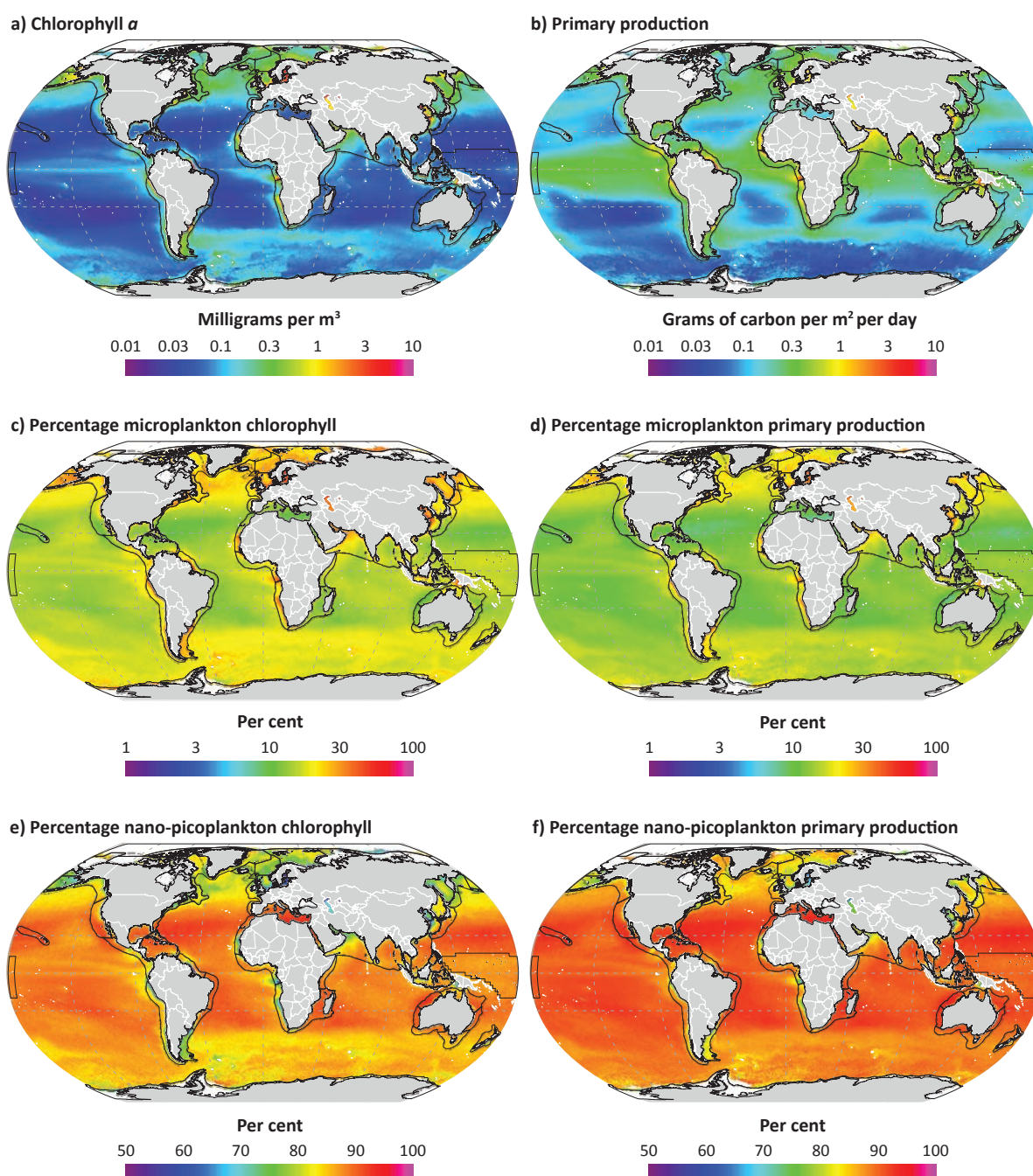
Figure 6.12 Distribution patterns for total chlorophyll a and primary production. Chlorophyll a and primary production estimates are shown first in total and then broken out into the microplankton and nano-picoplankton production estimates. These estimates of primary production enable estimates of high trophic level production to be modelled as the basis for understanding fishery productivity. High productivity is concentrated in upwelling regions. Primary production is dominated by nano-picoplankton production, especially in the deeper regions.
