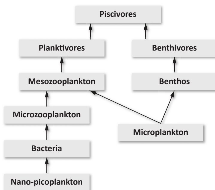
Figure 6.11 Food-web structure employed in this analysis. This structure specifically incorporates discrete components of meso, micro, and nano-picoplankton and bacteria. Nano-picoplankton, bacteria, and microzooplankton make up the microbial food web. This differs from classical representations that focus on microplankton. The classical grazing food web is fuelled by microplankton production. Species that shift their diets over an organism's lifespan and species with mixed feeding strategies can occupy multiple compartments in this representation.
