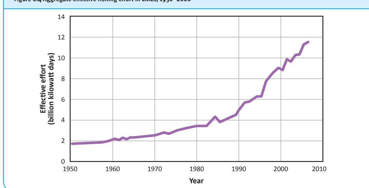
Figure 6.4 Aggregate effective fishing effort in LMEs, 1950–2006
