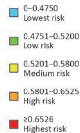
Sea-level Rise Threat Index
