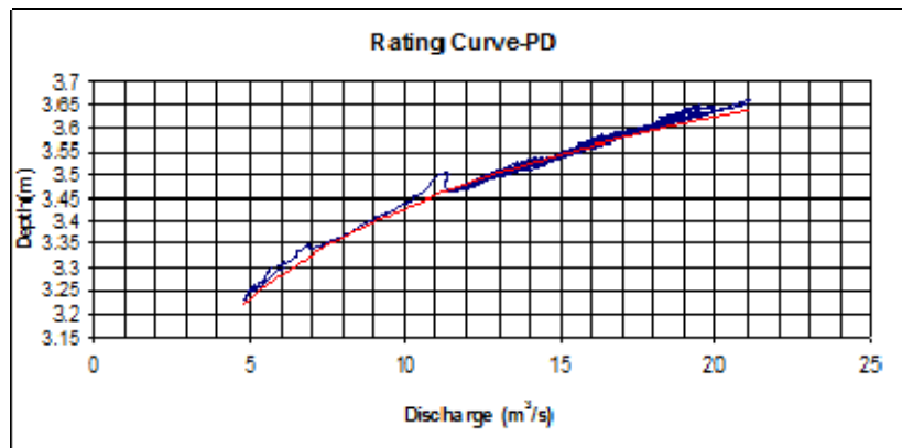
Figure 3-8 : Discharge - Depth Relationship – Xakanaka
